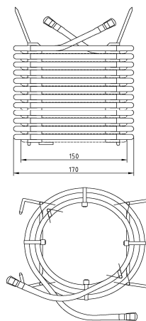
1serpentin/1 coil
